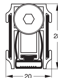
Stribo Acoustic Plus Anti-feu
